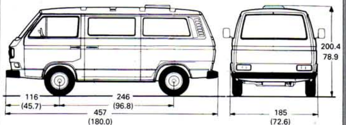
Exterior dimensions of Hi-Top
